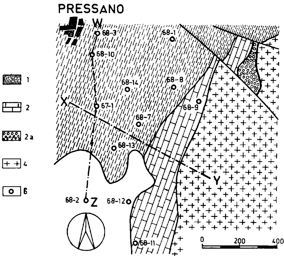
Fig. 5. Geological sketch map of the Lavis area
